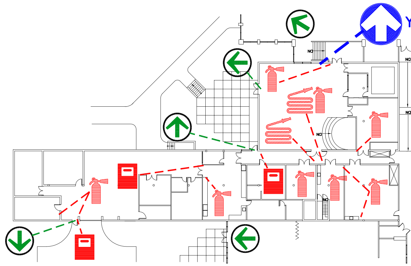
MPC8000 FLOOR PLAN (SE) LEVEL 10 NTS
