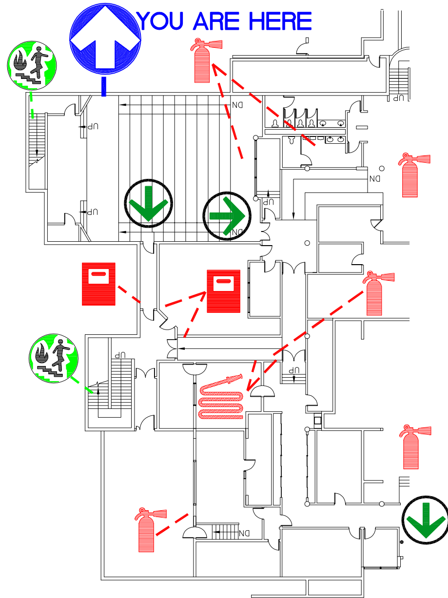
MPC7000 FLOOR PLAN (NE) LEVEL 09 NTS
