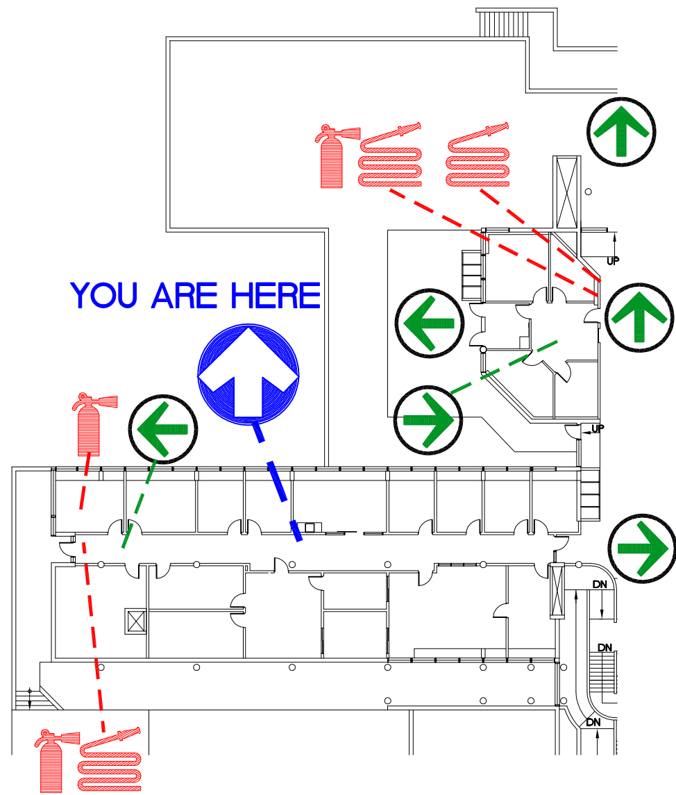
MPC8000 FLOOR PLAN (NW) LEVEL 10 NTS
